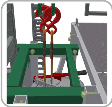
Dual wire rope system
