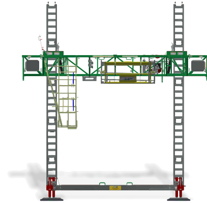
With standard walkway access system
