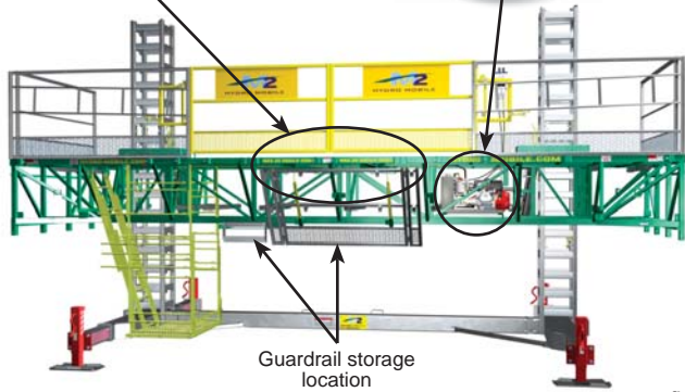
24' (7,3 m) motorized unit shown in this illustration
