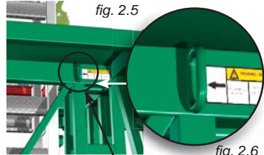
fig. 2.5 Tie a lifeline with a rope grab or a self-retracting lifeline to the designated tie point under the motorized unit
